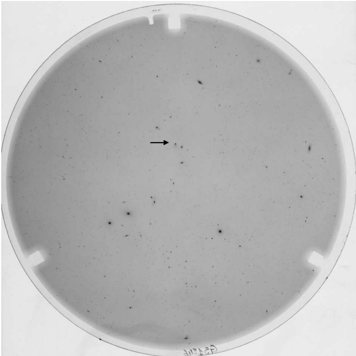
Fig. 36: Discovery plate of Comet 1972VIII/1973a (arrow) taken on 11 January 1973 at the IALg-CNRS Big Schmidt telescope during an observing run with students at Haute Provence Observatory (cf. pp. 50ff and publications listed). The field selected was the dense Virgo cluster of galaxies, making a comet identification particularly not obvious, as confirmed by several post-discoveries. The episode was particularly exciting for the students. See also Fig. 38 & 219.
