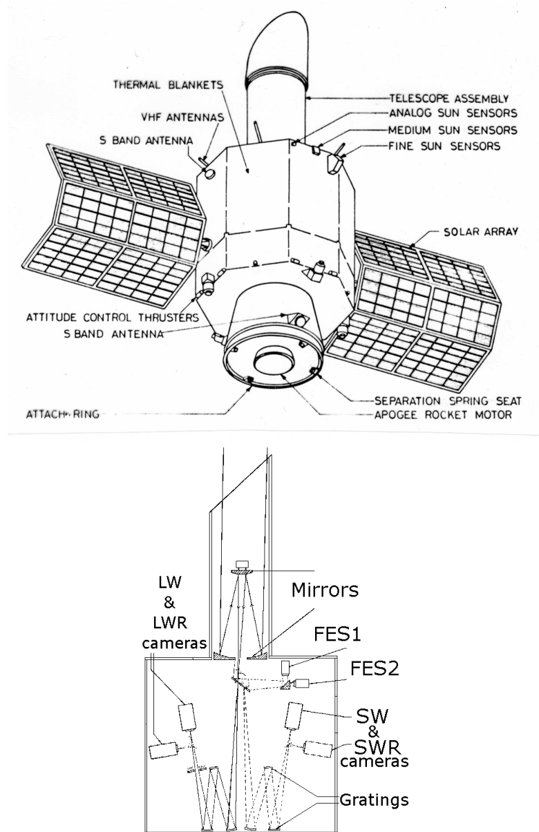
Fig. 66: The major IUE components are pointed out in these schematic views. The Ritchey-Chrétien telescope had a 45cm mirror open at f/15 and provided 3'' images in a 16' field. The wavelength range covered was 1150\text{--}3200\text{\AA} splitted between short wavelength (SW, \sim 1150\text{--}2000\text{\AA} ) and long wavelength (LW, \sim 1900\text{--}3200\text{\AA} ), in each case with a prime (P) and a redundant (R) camera. There were two resolution modes: low dispersion ( \sim 6.1\text{\AA} for SW and \sim 9.2\text{\AA} for LW) and high dispersion via an echelle grating ( \sim 0.1\text{\AA} for SW and \sim 0.2\text{\AA} for LW). Two entrance slits could be used for the spectrograph: a \sim 3'' circle (50% throughput for point sources) and an \sim 10'' \times 20'' oval. The Fine Error Sensors (FES) were used for guidance. In short, beyond its much more flexible exploitation ( à-la-carte observing versus survey), IUE covered a larger wavelength range than TD1 and, even at low dispersion, its resolution was about five times better.
