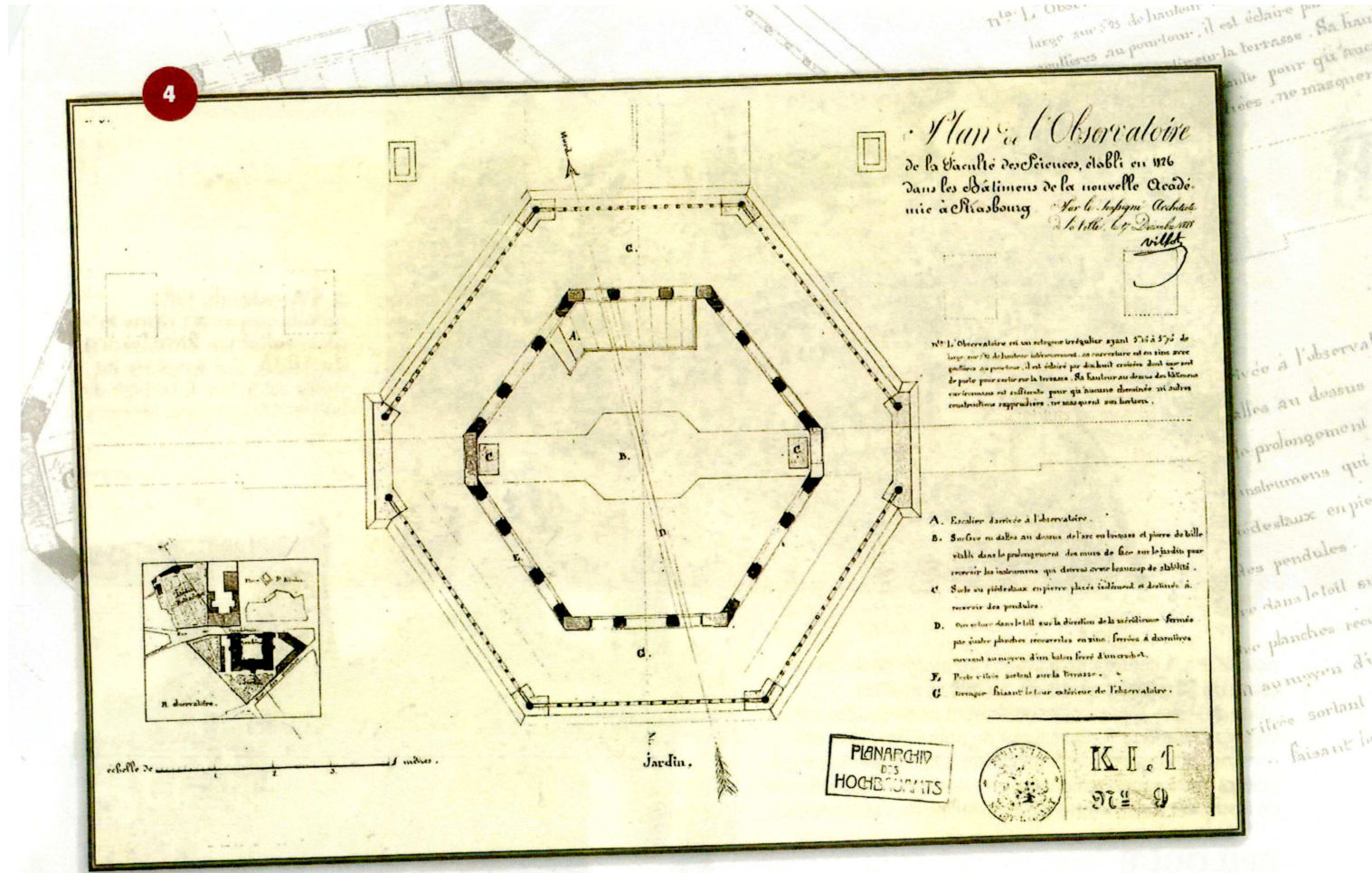
Fig. 181: One of the gold nuggets found by Heck in the local archives is this floor plan for Strasbourg 19 th -century Academy observatory as reproduced here from Publ. 667. It is dated 17 December 1828 and was drawn by Architect Jean-Nicolas Villot. (Courtesy AVCUS & SAF)
