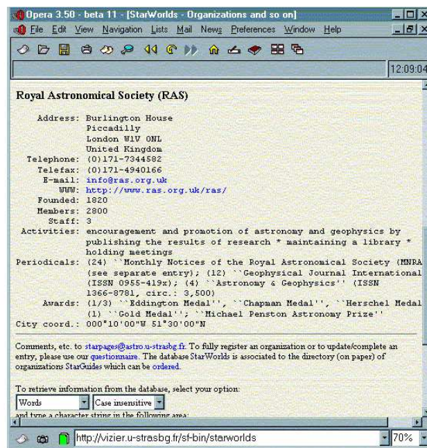
Fig. 143: StarWorlds query for "Royal Astronomical Society" on an earlier web navigator (Netscape) and the result of the same query on another one (Opera).
