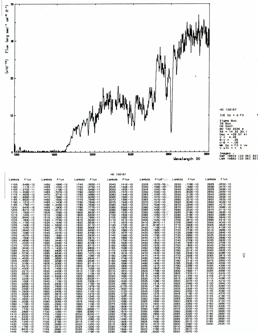
Fig. 106: Example of inside pages from the "IUE Low-Dispersion Spectra Reference Atlas. Part 1. Normal Stars" (Publ. 413) displaying the spectrum and flux table for the star HD128167 ( \sigma Boo), an F3 dwarf.
