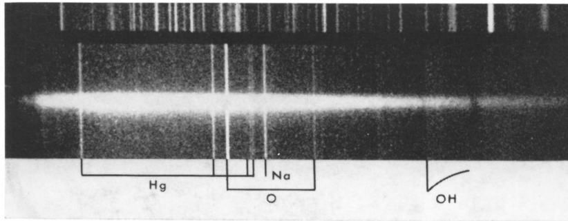
Fig. 219: Comet 1972VIII/1973a was discovered in January 1973 by our biographeer when observing with the Big Schmidt telescope at Haute Provence Observatory (OHP). Refer to p. 50 for the story and to Fig. 36 for the discovery field. First comet discovered at OHP, the object was then of magnitude 12 and moving away at about 2.2 AU from the Earth and about 2.7 AU from the Sun. The spectrum above has been obtained at the 193cm OHP telescope. It shows a continuum from 3700Å in the violet (left) to 8700Å in the near infrared. Mercury and sodium emissions are due to city lighting; oxygen and hydroxyl ones are from the night sky. (© Sky & Telescope, May 1973)
