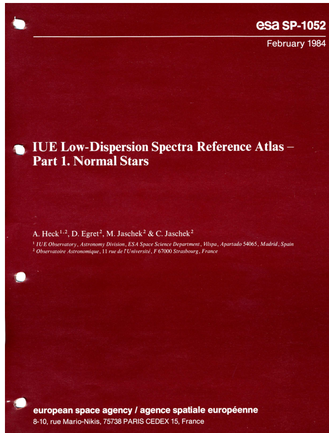
Fig. 105: Cover page of the IUE low-dispersion spectra reference atlas (Publ. 413).
