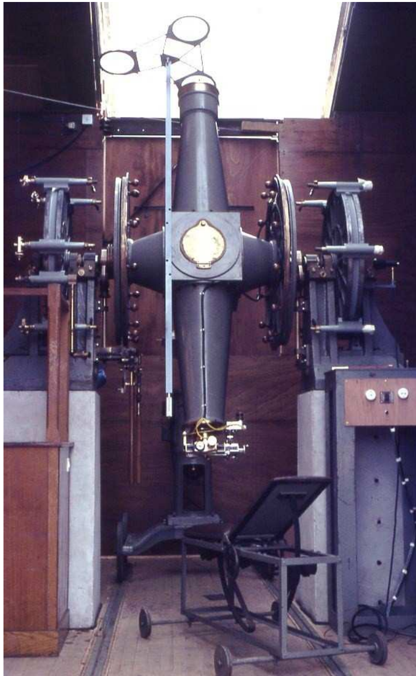
Fig. 28: The Liège meridian instrument is seen here in its Belloch shelter. Delivered and installed in Liège in 1931-1932 by the Parisian firm Gautier-Prin, it has a 19cm objective lens with a 2.35m focal length. The optics is signed André Couder. (Courtesy J.M. Rousseau)
