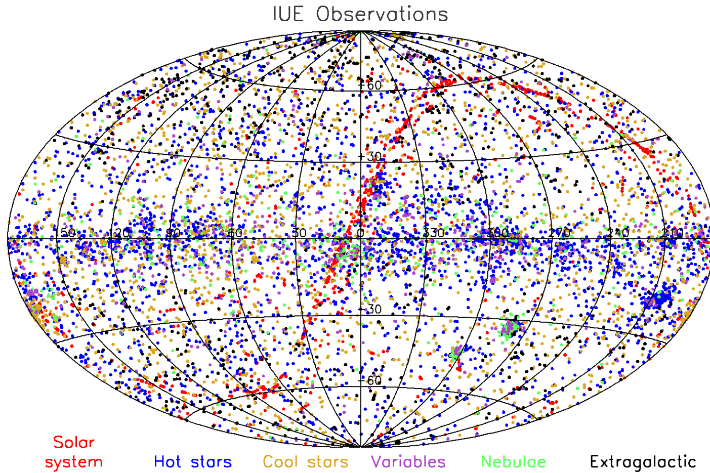
Fig. 93: Celestial distribution of IUE observations in galactic coordinates ( 0^\circ at center) from the "Final Merged Log of IUE Observations" (NASA-ESA 2000). (Graphism by L. Cambr sy)
