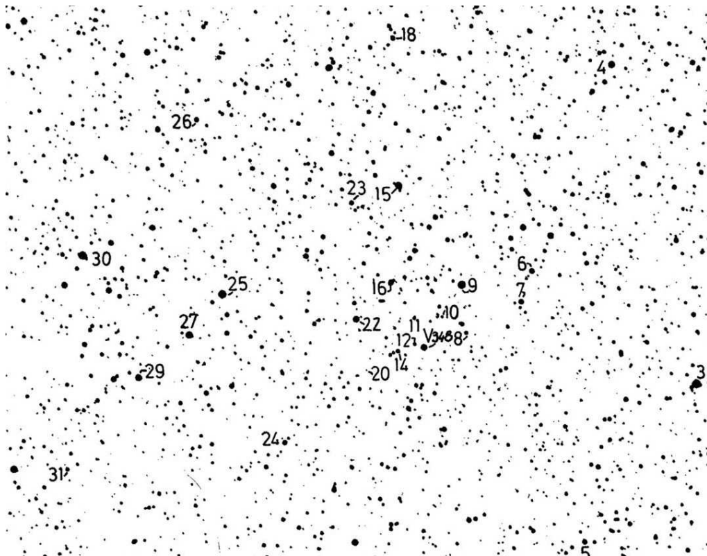
Fig. 109: The crowded field of V348 Sgr can explain numerous pointing mistakes and incorrect interpretations by some observers, especially since the object can suddenly become much fainter and even invisible in some instruments. (Reproduced from Publ. 60)
